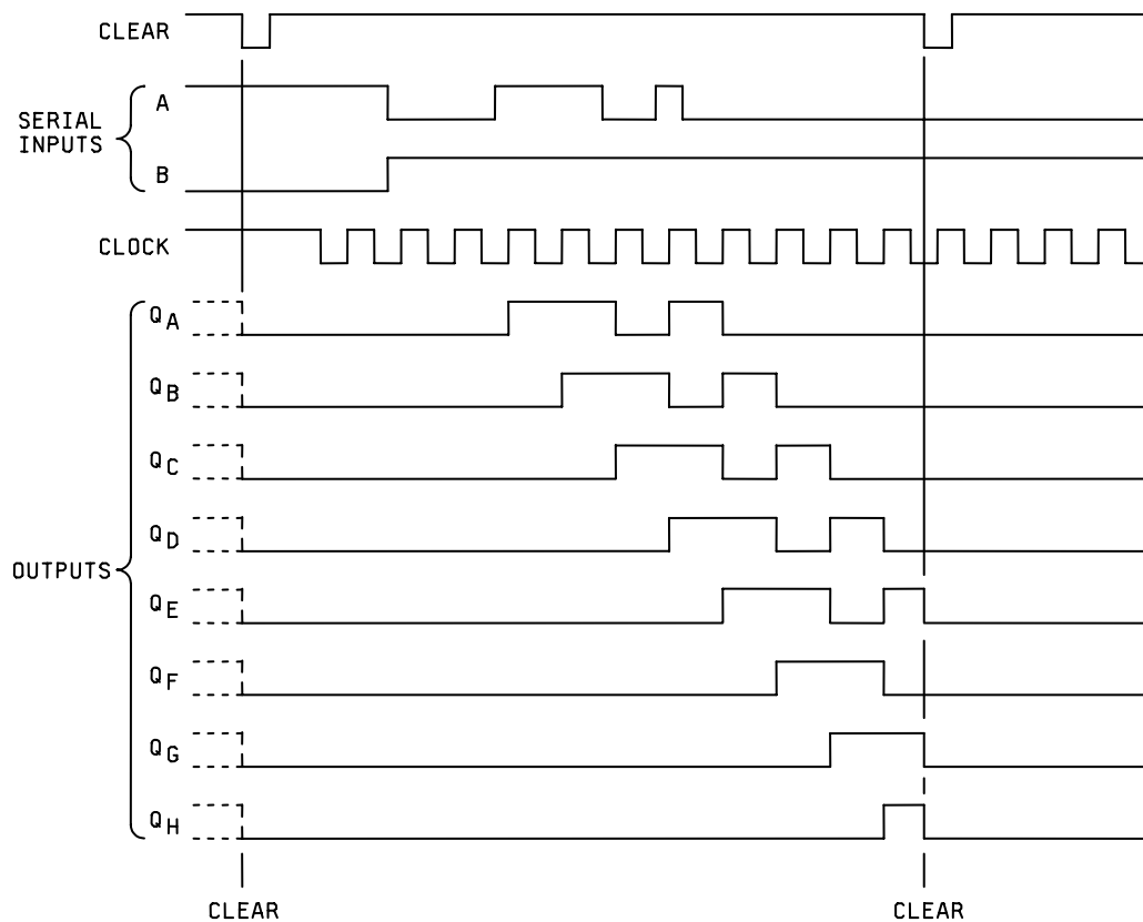
TYPICAL CLEAR,INHIBIT,SHIFT,CLEAR AND INHIBIT SEQUENCES
