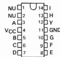
SN54H54 . . . W PACKAGE
