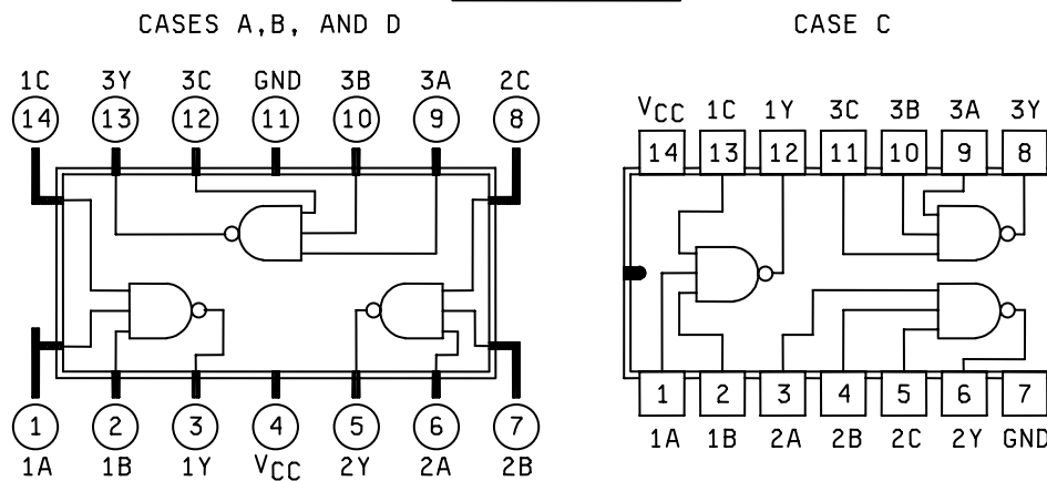
Figure 1. Logic diagrams and terminal connections (top view).
