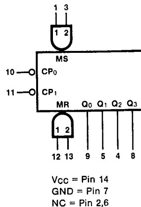
LOGIC SYMBOL
