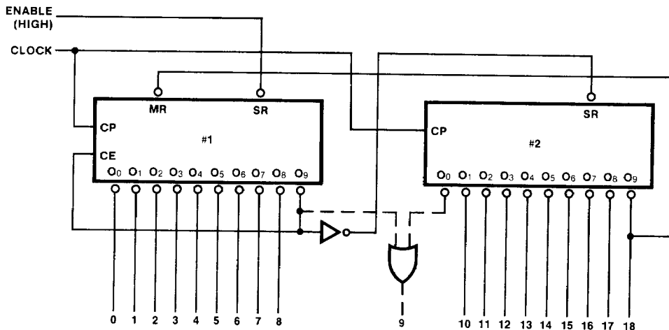
Fig. c Expansion for longer sequences. The first sequencer locks up after \bar{O}_9 goes LOW because of the feedback to CE. Simultaneously, \bar{S}R of the second sequencer is released and it starts counting on the next clock. When \bar{O}_9 of the second sequencer goes LOW, the feedback to \bar{M}R causes \bar{O}_9 of the first sequencer to go HIGH, which then makes \bar{S}R of the second sequencer go HIGH. On the next clock the second sequencer goes to the \bar{O}_0 state, releasing \bar{M}R of the first sequencer, making its \bar{O}_0 go LOW. On the next clock the first sequencer starts its counting sequence again.
