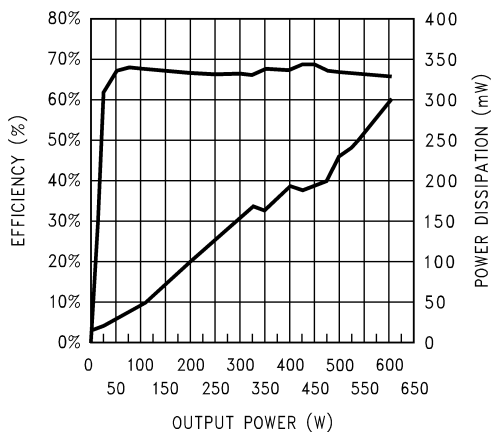
Efficiency (top trace) and Power Dissipation (bottom trace) vs Output Power V_{DD} = 3.3V , R_L = 4\Omega + 33\mu H , f = 1kHz , THD < 2%
