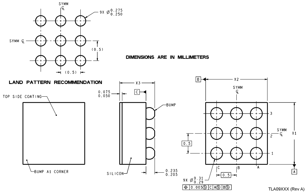
9 Bump micro SMD Order Number LM4665ITL, LM4665ITLX NS Package Number TLA09AAA X 1 = 1.514 X 2 = 1.514 X 3 = 0.600
