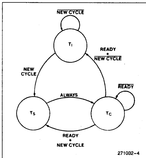
Figure 4. M82289 Processor Bus States
