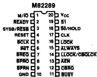
Figure 2. M82289 Pin Diagram
