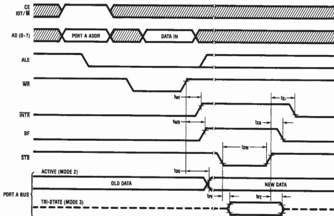
Strobed Mode Output
