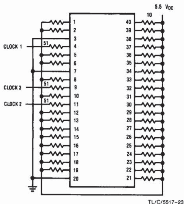
5242HR NSC810AD/883B (Dual-In-Line)
