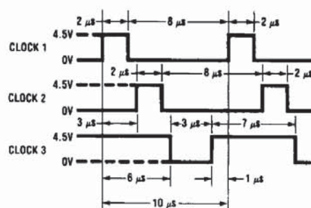
Input Clocks
