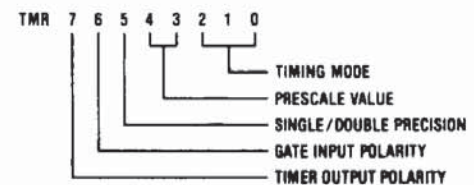
FIGURE 4. Timer Mode Register
