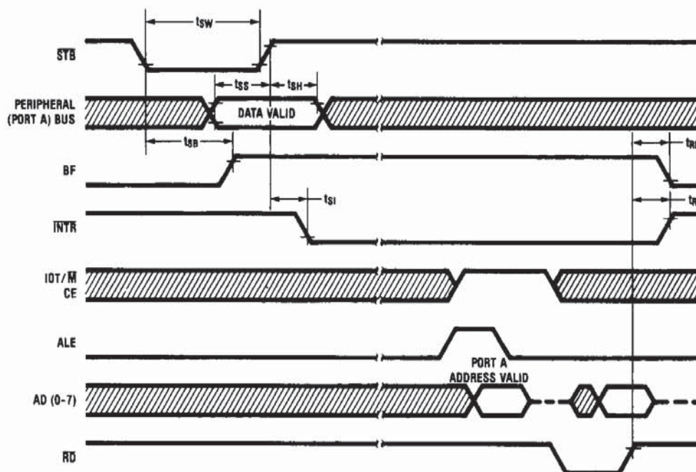
Strobed Mode Input
