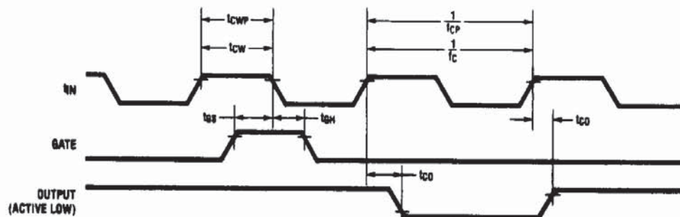
Timer Waveforms
