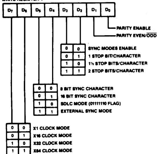
Figure 10. Write Register Bit Functions (Continued)
