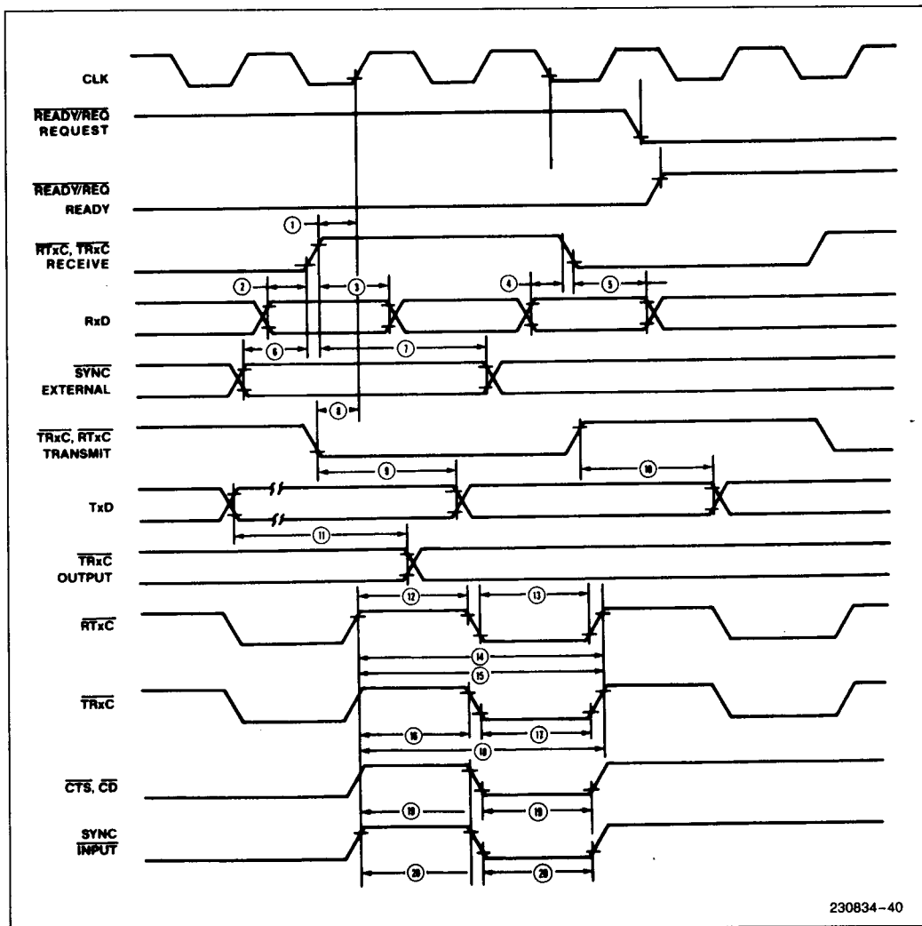
Figure 18. General Timing
