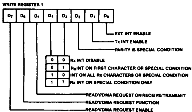
Figure 10. Write Register Bit Functions
