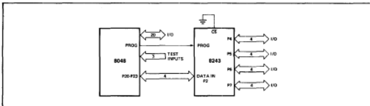
Figure 4. Expander Interface
