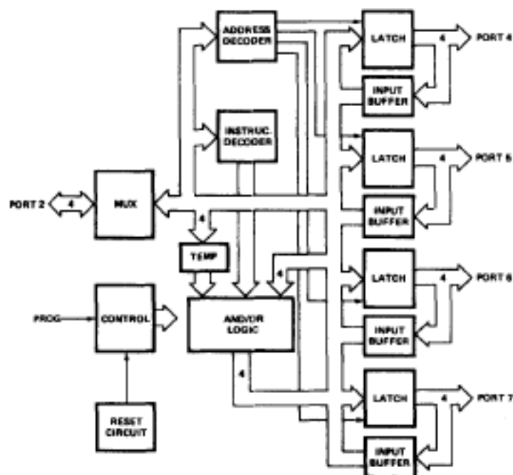
Figure 1. 8243 Block Diagram
