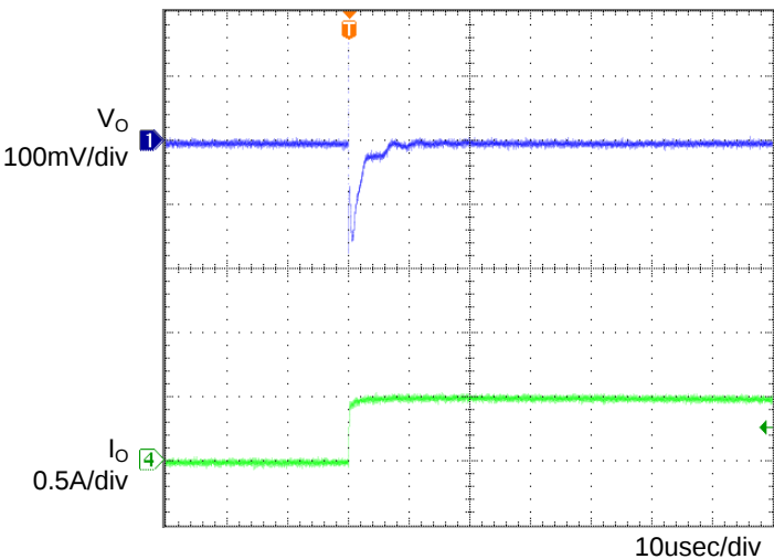
Figure 3. Transient Response (0→0.5A) Co=1 \mu F, Ta=-40°C
