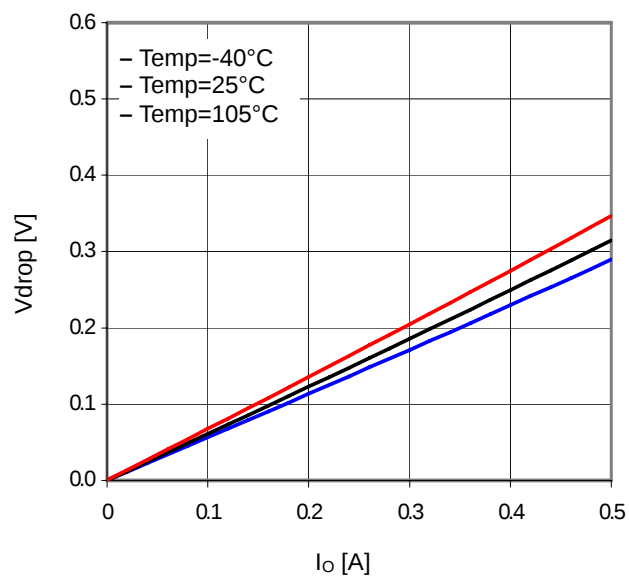
Figure 35. Minimum dropout Voltage 2 ( V_{CC}=6.0\text{V} )
