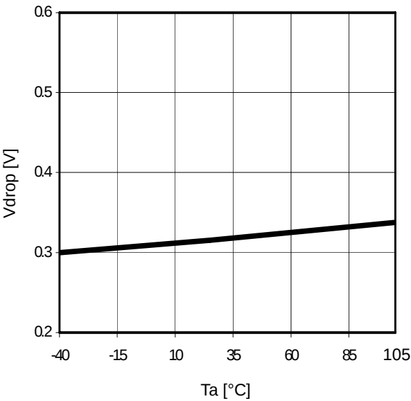
Figure 33. T a -V drop (V CC =6V, I o =0.5A)
