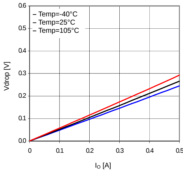
Figure 36. Minimum dropout Voltage 3 ( V_{CC}=8.0\text{V} )
