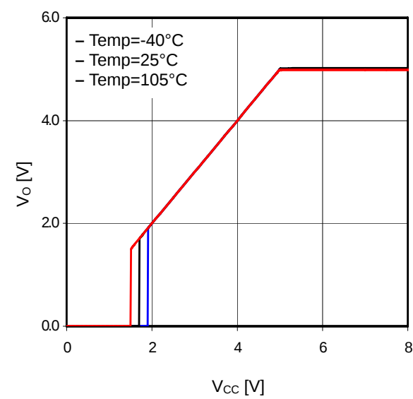
Figure 27. V_{CC}-V_o ( I_o=0mA )
