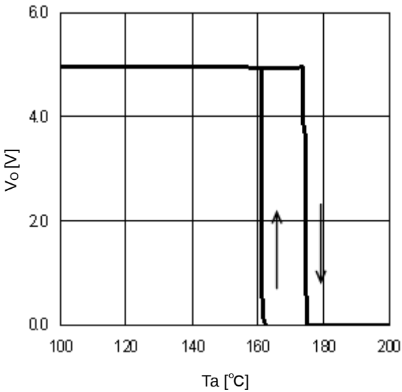
Figure 28. TSD ( I_o=0mA )
