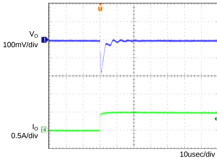
Figure 5. Transient Response (0→0.5A) Co=1 \mu F, Ta=105°C
