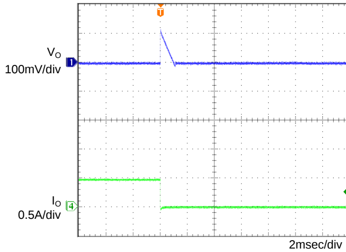
Figure 6. Transient Response (0.5→0A) Co=1 \mu F, Ta=-40°C
