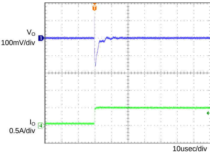
Figure 4. Transient Response (0→0.5A) Co=1 \mu F, Ta=25°C
