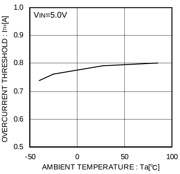
Figure 13. Over-current threshold
