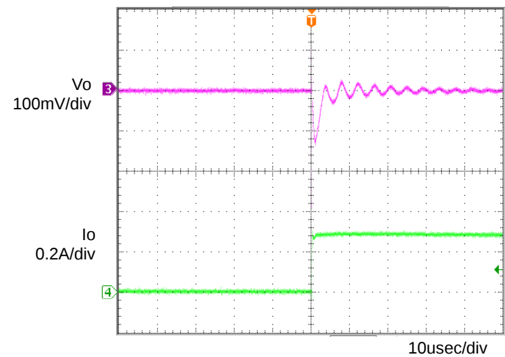
Figure 3. Transient Response (0→0.3A) Co=1 \mu F, Ta=-40°C
