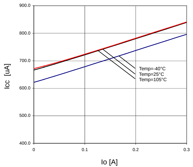
Figure 30. I_o - I_{CC}
