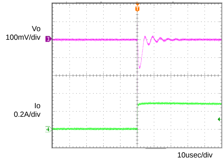
Figure 5. Transient Response (0→0.3A) Co=1 \mu F, Ta=105°C
