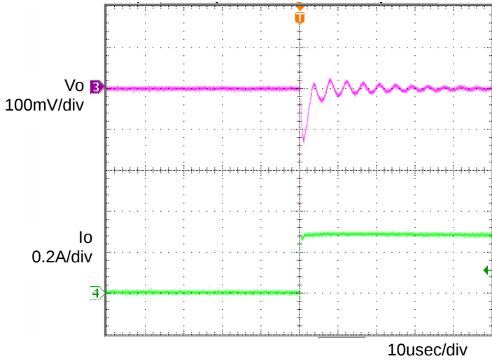
Figure 4. Transient Response (0→0.3A) Co=1 \mu F, Ta=25°C
