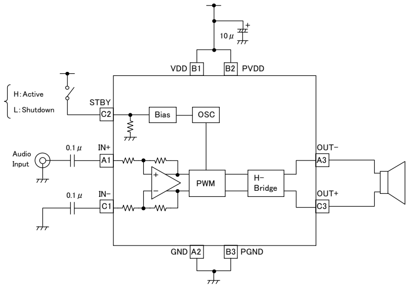
Fig.3 Single-Ended input
