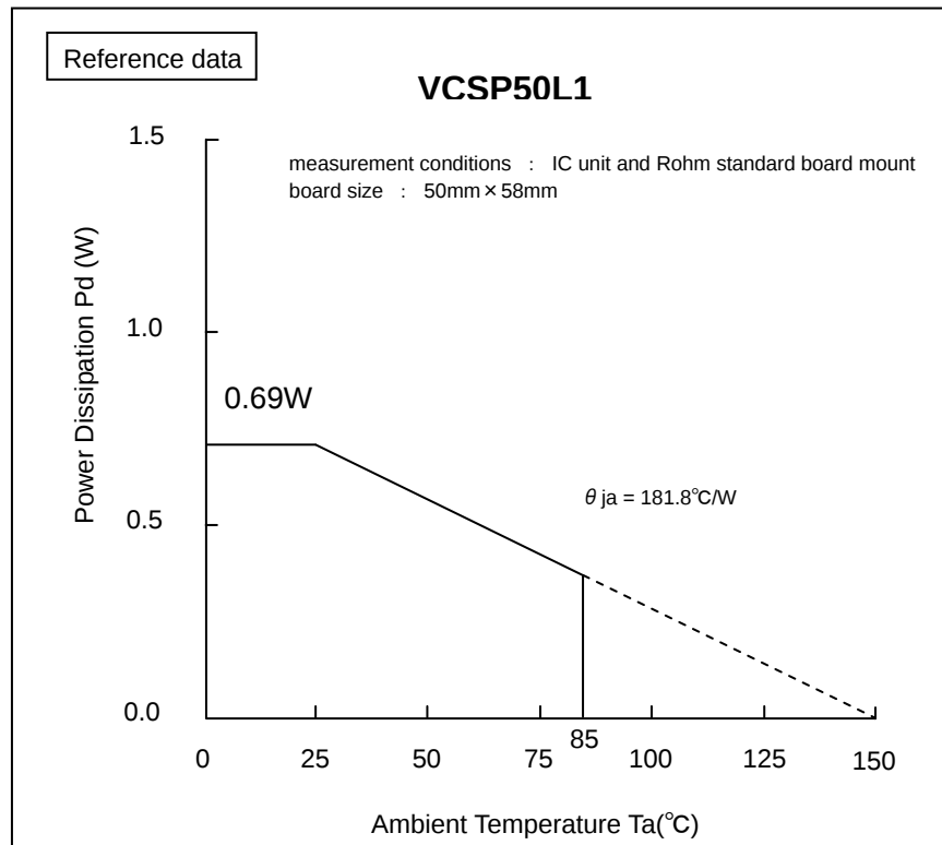
Temperature Derating Curve
