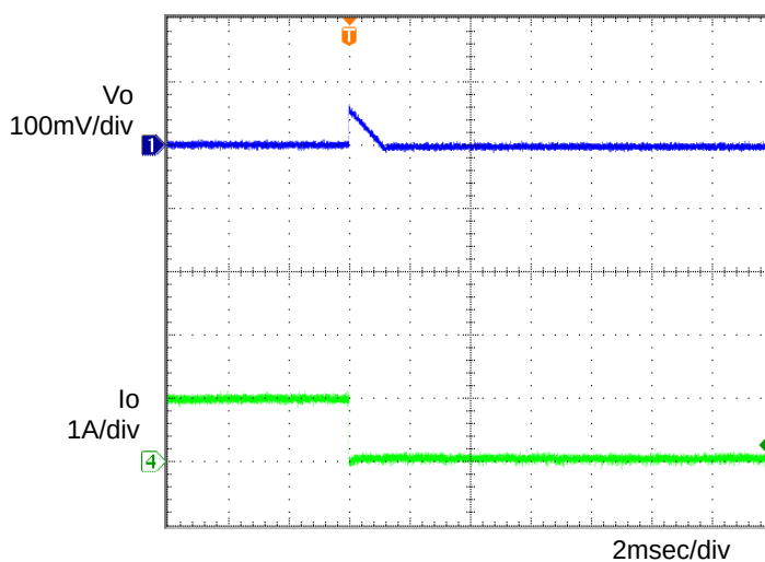
Figure 6. Transient Response (1.0→0A) C_o=1\mu\text{F} , T_a=-40^\circ\text{C}
