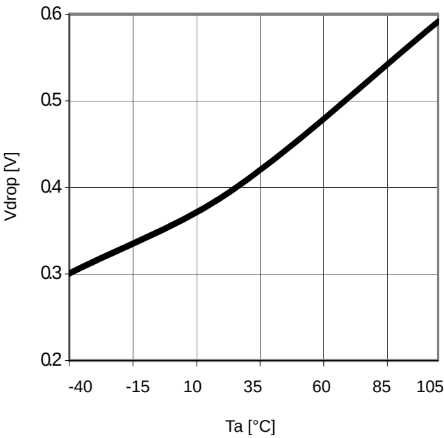
Figure 33. T_a - V_{drop} ( V_{CC}=6V , I_o=1A )
