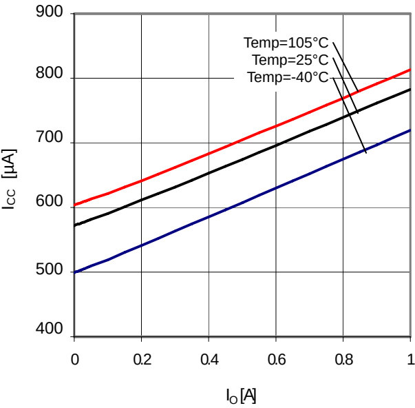
Figure 30. I_O-I_{CC}
