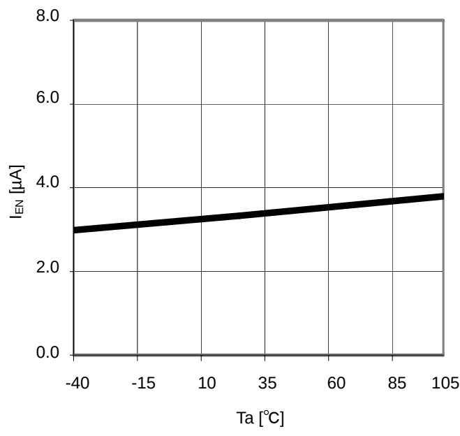
Figure 24. T_a - I_{EN}
