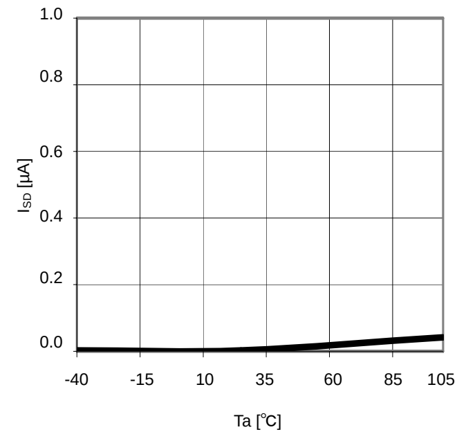
Figure 23. T_a - I_{SD} ( V_{EN}=0\text{V} )
