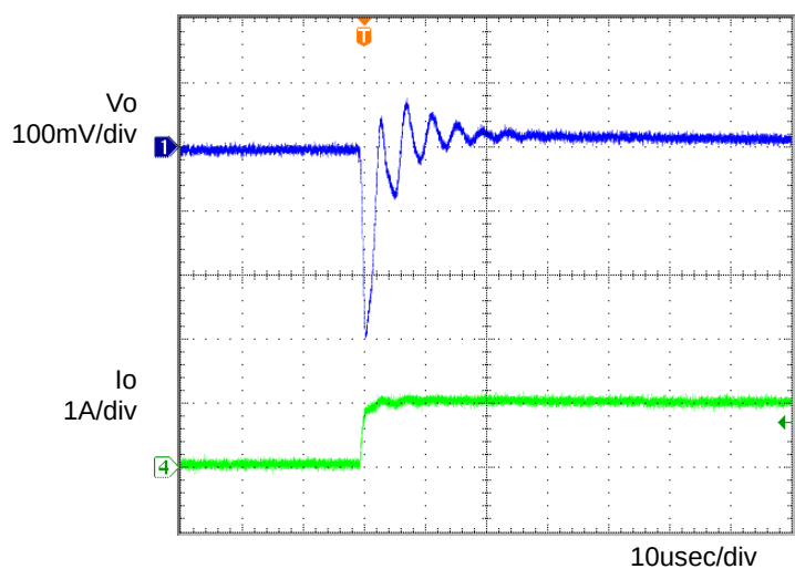
Figure 5. Transient Response (0→1.0A) C_o=1\mu\text{F} , T_a=105^\circ\text{C}
