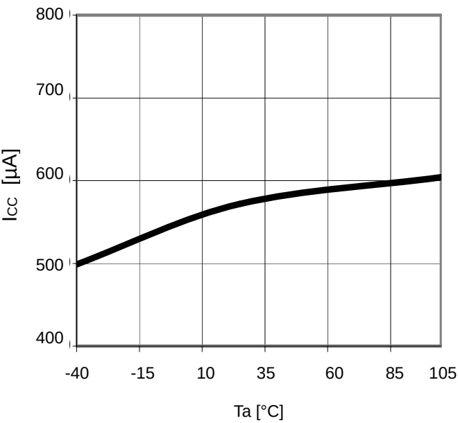
Figure 22. T_a - I_{CC}
