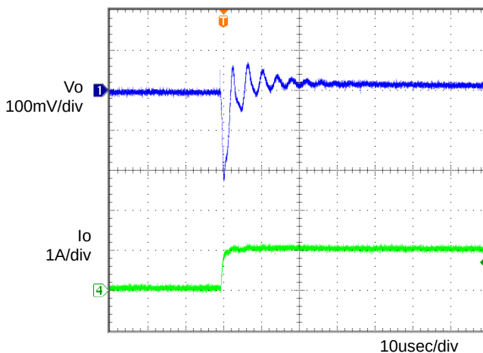
Figure 4. Transient Response (0→1.0A) C_o=1\mu\text{F} , T_a=25^\circ\text{C}
