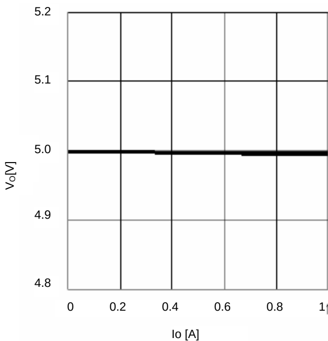
Figure 25. I_O - V_O
