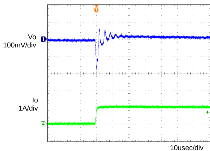
Figure 3. Transient Response (0→1.0A) C_o=1\mu\text{F} , T_a=-40^\circ\text{C}
