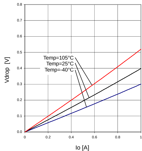
Figure 35. Minimum dropout Voltage 2 (V CC =6.0V)
