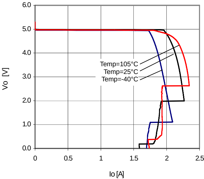
Figure 29. OCP
