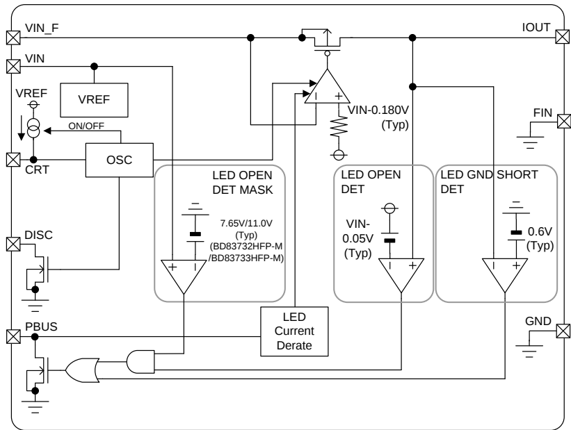
Figure 3. Block Diagram
