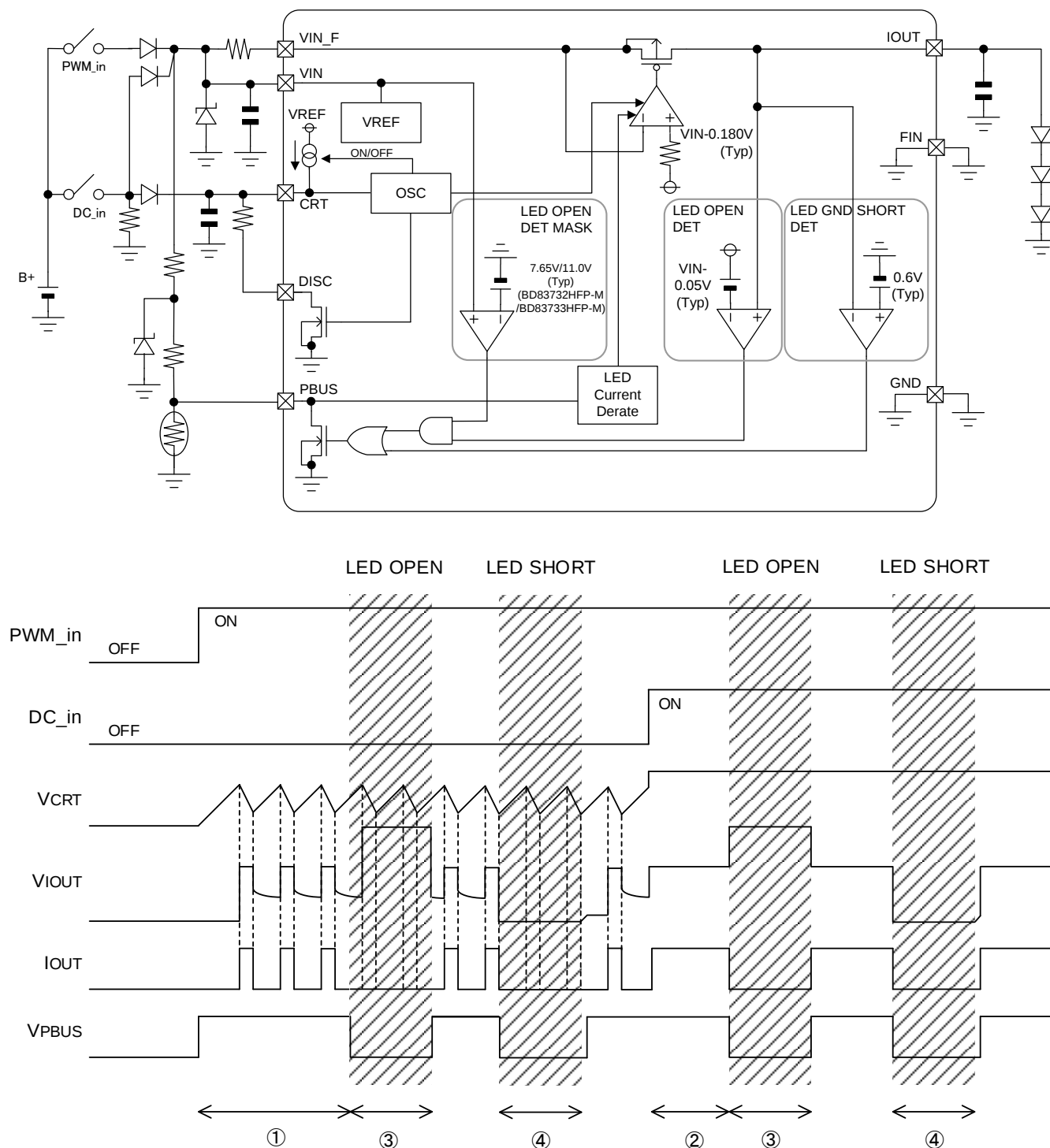
Figure 28. Timing Chart
