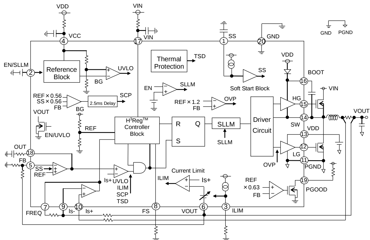
Figure 3. Block Diagram
