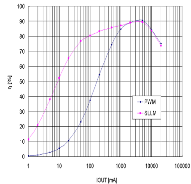
Figure 4. Efficiency ( V_{IN}= 7.5V )
