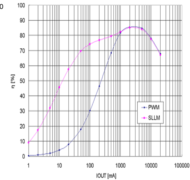
Figure 6. Efficiency ( V_{IN}= 21V )
