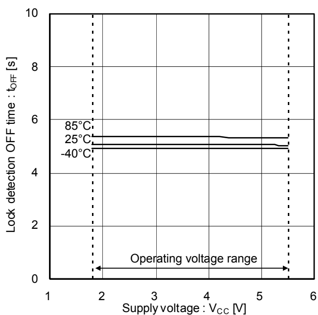
Figure 18. Lock Detection OFF Time
