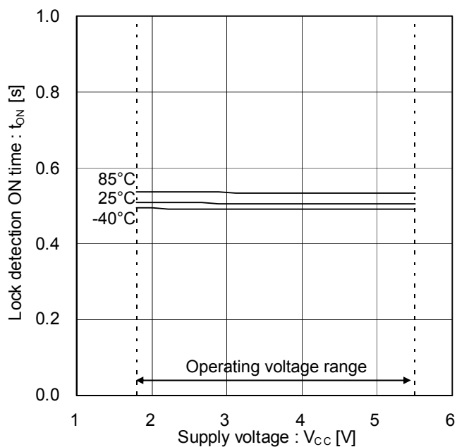
Figure 17. Lock Detection ON Time
