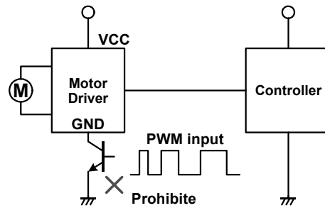
Figure 30. GND Line PWM switching prohibited
