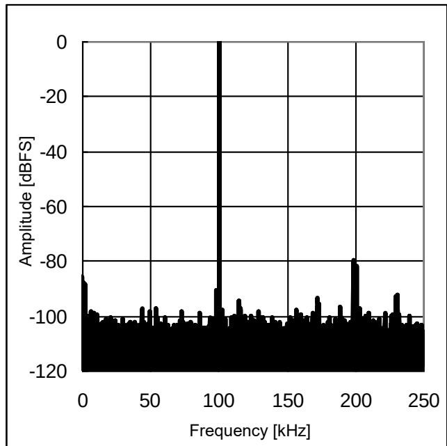
Figure 12. Amplitude vs Frequency ( V_A = 5\text{ V} , f_{\text{SCLK}} = 10\text{ MHz} , f_s = 500\text{ kSPS} )
