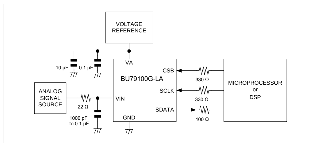
Figure 20. Application Circuit
