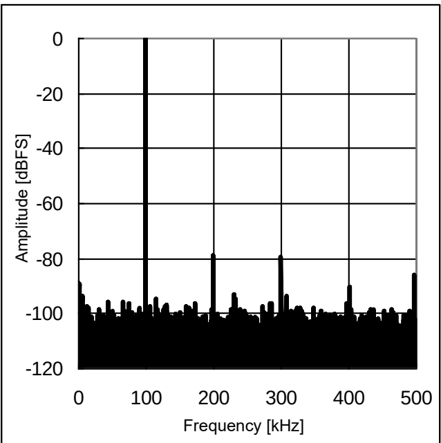
Figure 13. Amplitude vs Frequency ( V_A = 5\text{ V} , f_{\text{SCLK}} = 20\text{ MHz} , f_s = 1\text{ MSPS} )
