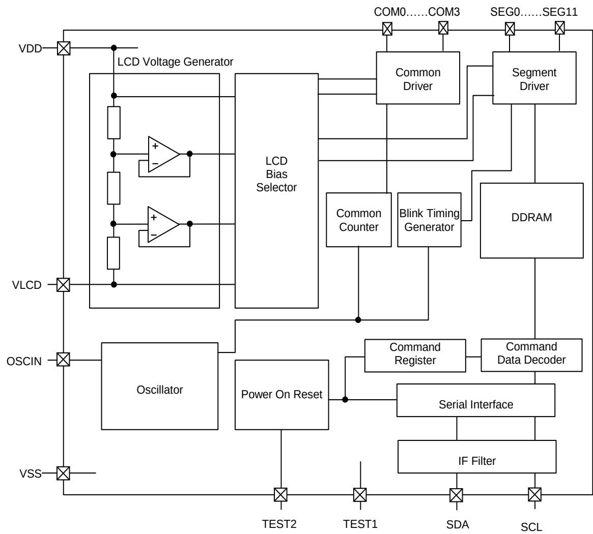
Figure 2. Block Diagram
