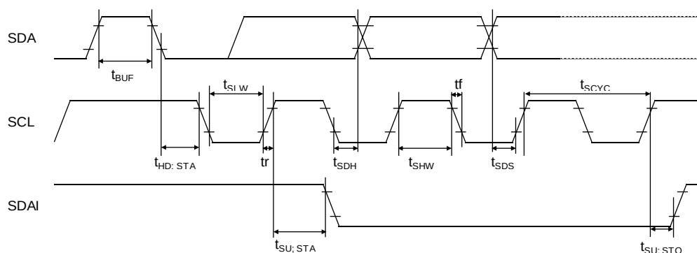
Figure 5. Interface Timing
