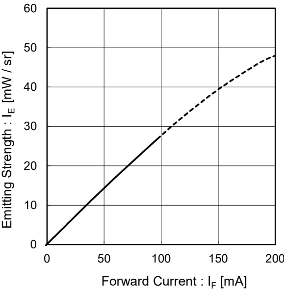
Fig.3 Emitter Strength vs. Forward Current
