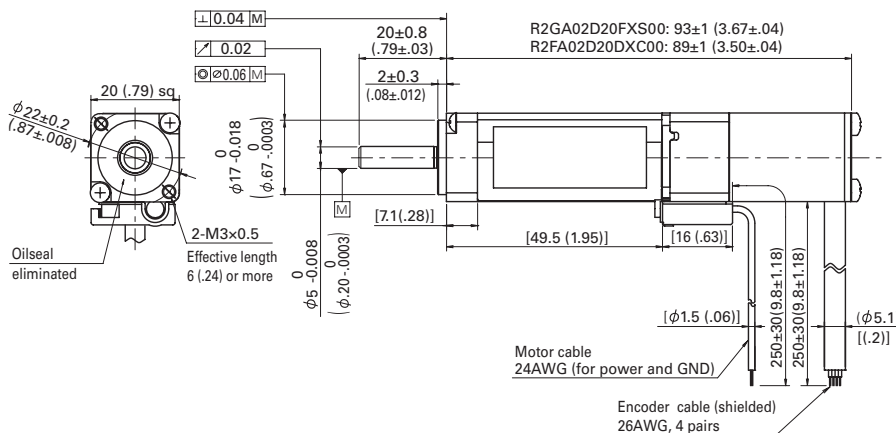
Encoder Dimensions for R2FA02D20DXC00
