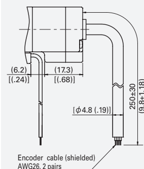
Encoder Dimensions for R2FA02D20DXC00
