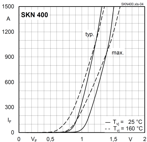
Fig. 5 Forward characteristics
