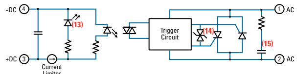
Diagram: Series 1 DC control
