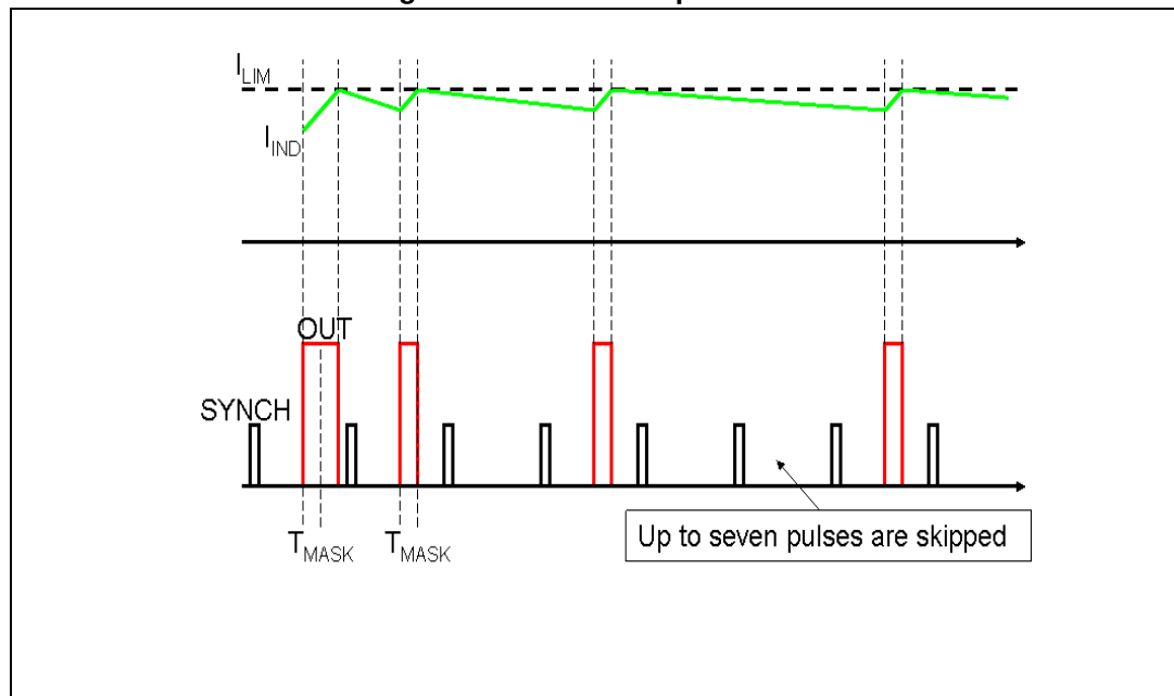
Figure 8. Overcurrent protection
