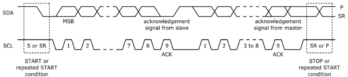
Figure 21. Bit transfer
