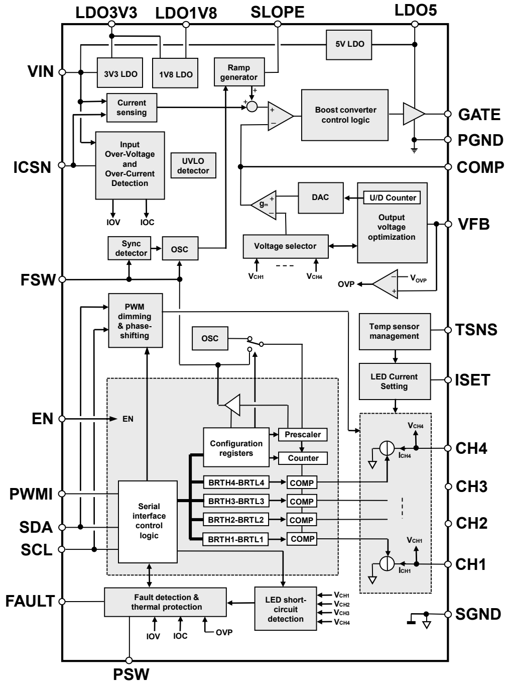
Figure 1. Block diagram
