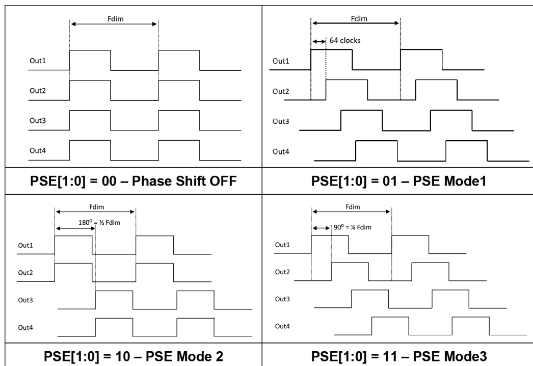
Figure 12. Output signal vs. phase shift modes
