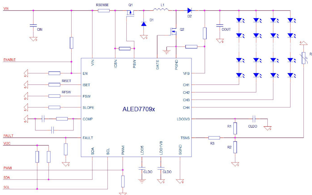
Figure 3. Example of boost topology application with I 2 C and PWMI control
