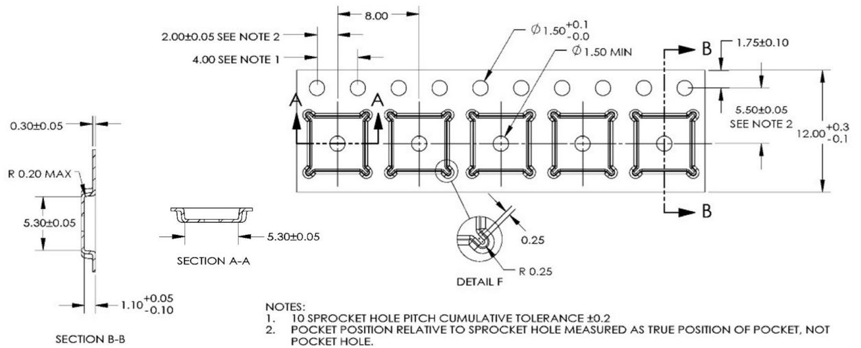
Figure 30. QFN24L (5x5 mm) carrier tape outline (dimensions are in mm)
