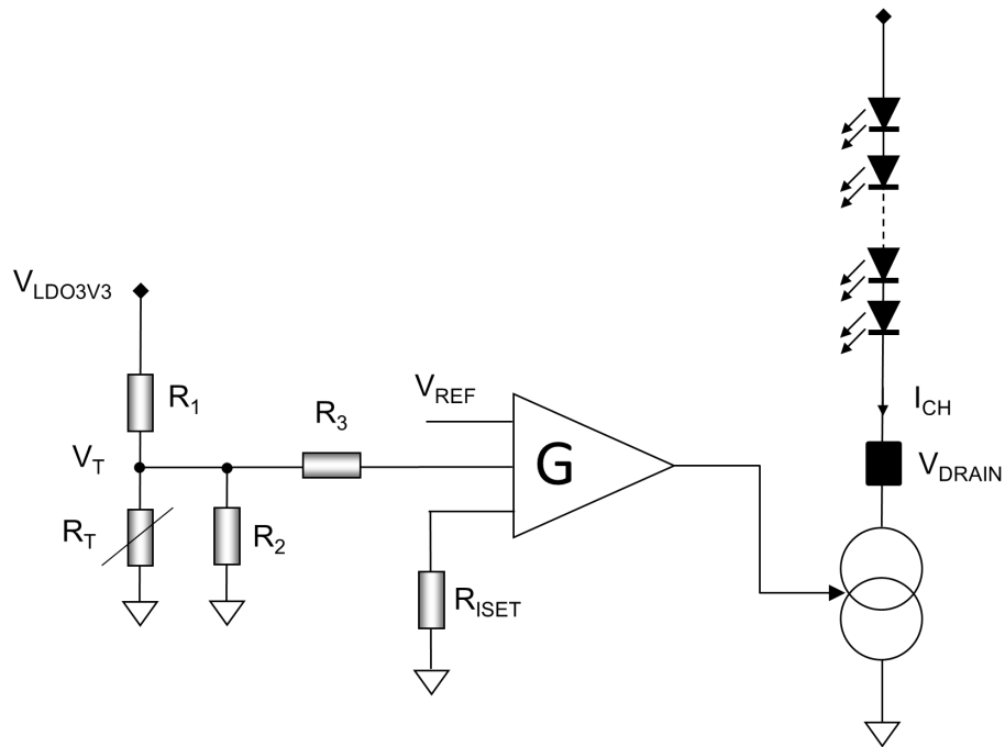
Figure 17. Temperature control circuit
