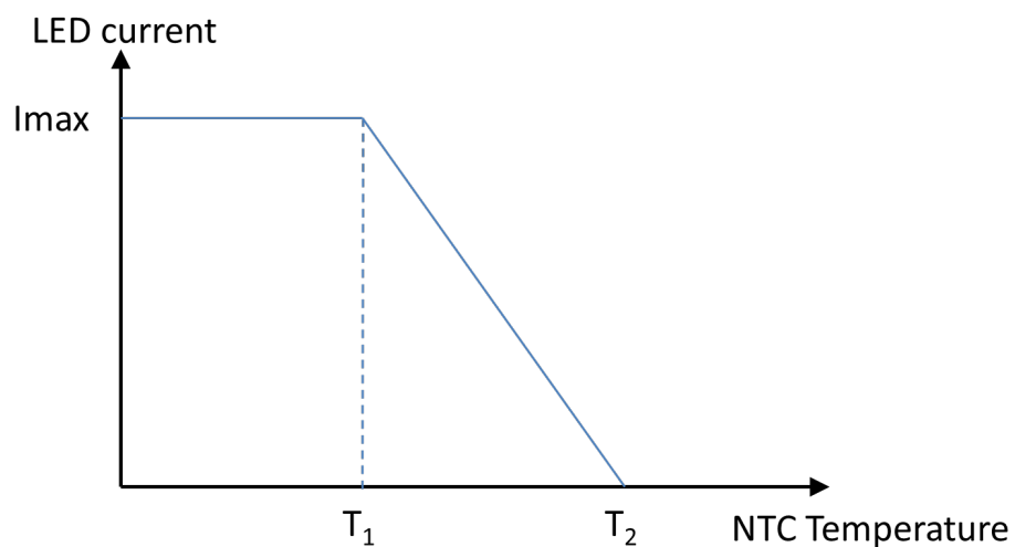
Figure 16. Current control by NTC
