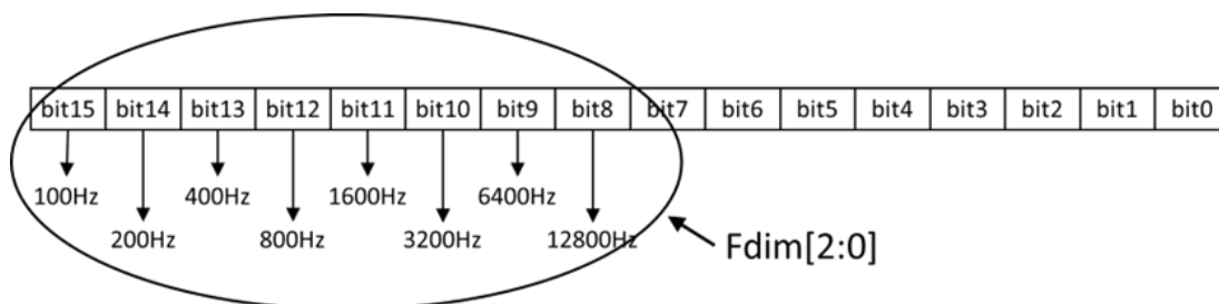
Figure 13. Number of bit vs. Fdim
