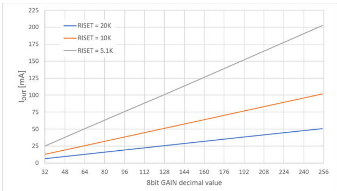
Figure 11. I_{OUT} linearity with GAIN at different R_{ISET}
