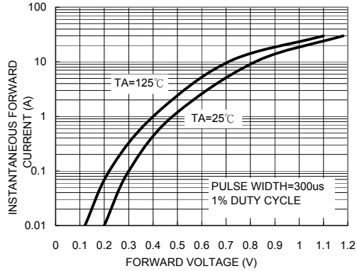
FIG.3- TYPICAL INSTANTANEOUS FORWARD CHARACTERISRICS PER LEG
