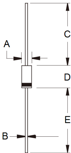
DO-204AC (DO-15)
