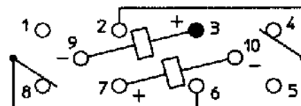
TERMINAL VIEW
