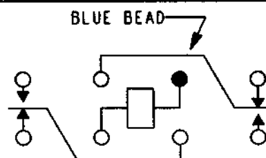
TERMINAL VIEW
