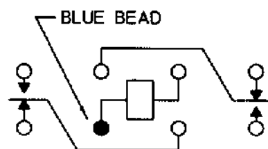
TERMINAL VIEW
