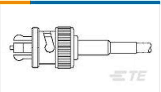
TE Part #5051426-2 SAFE HIGH VOLTAGE PLUG
