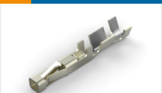
TE Part #1-794606-3 MICRO MNL RPT CNT STRP 30AU LF
