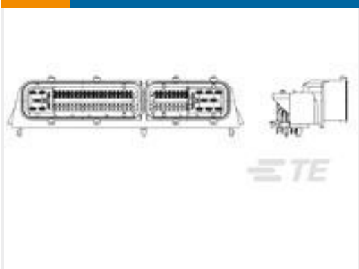
TE Part #1241434-1 121pos hybrid MQS .63 header 90deg
