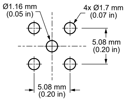
Figure 2. Recommended PCB Dimensions for the CONSB001-1-G
