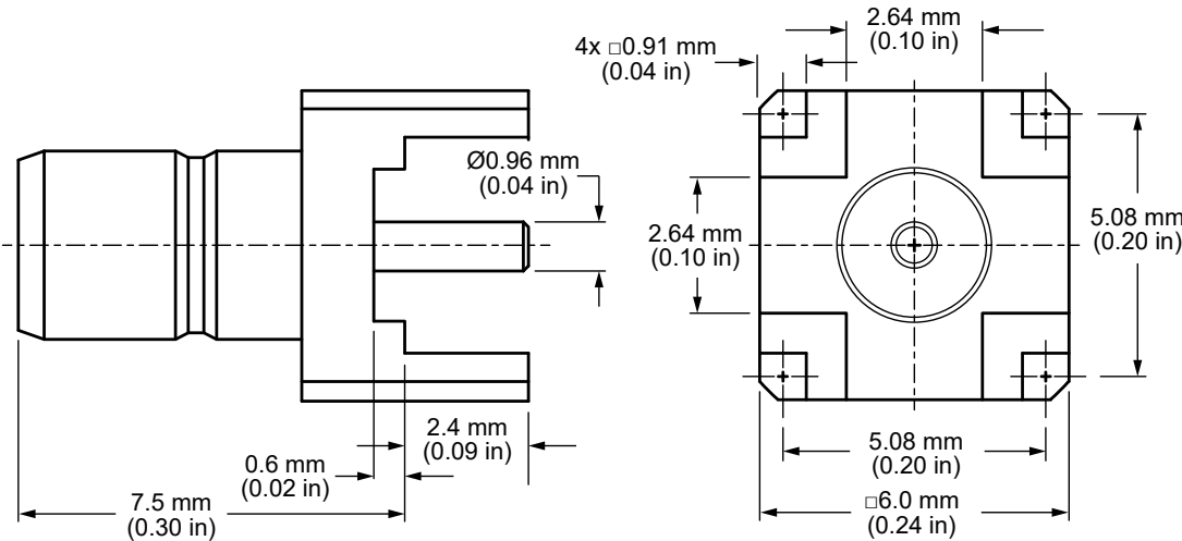
Figure 1. Product Dimensions for the CONSMA024-G Connector
