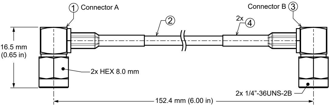
Figure 1. Product Dimensions for the CSE-SGMR-152-SGMR Cable Assembly
