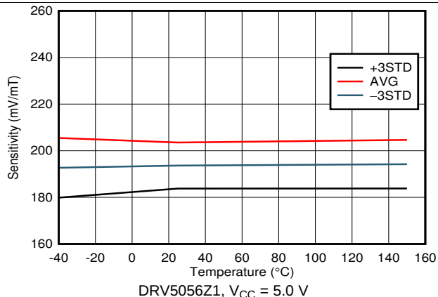
Figure 20. Sensitivity vs Temperature
