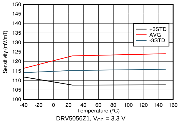
Figure 19. Sensitivity vs Temperature
