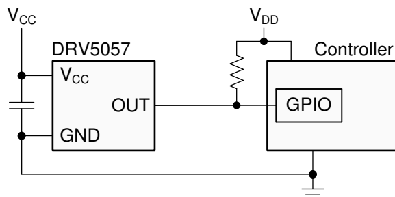
Typical Schematic
