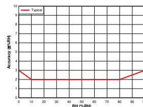
RH Accuracy
