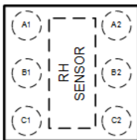
Figure 5-1. WLCSP (DSBGA) 6-Pin YPA Top View
