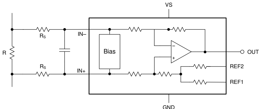
Figure 9-1. Filter at Input Pins
