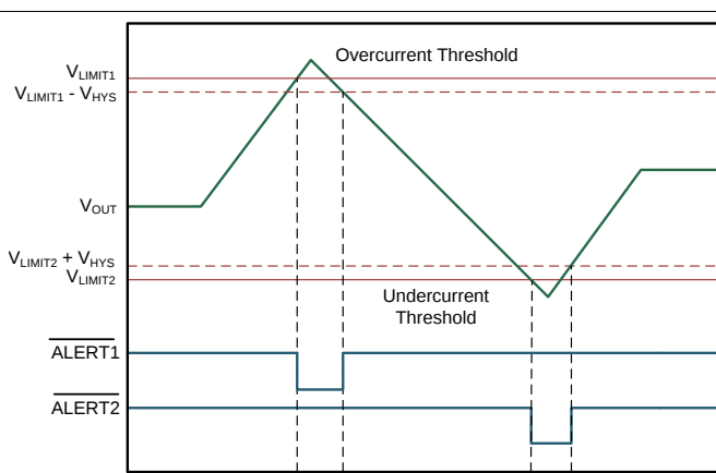
Figure 46. Comparator Hysteresis Behavior (INA303)
