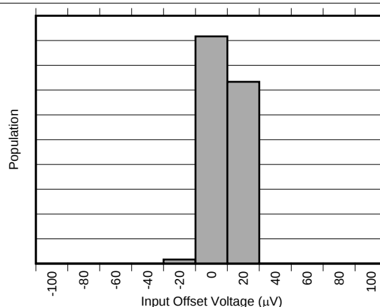
Figure 2. Input Offset Voltage Distribution (INA30xA2)
