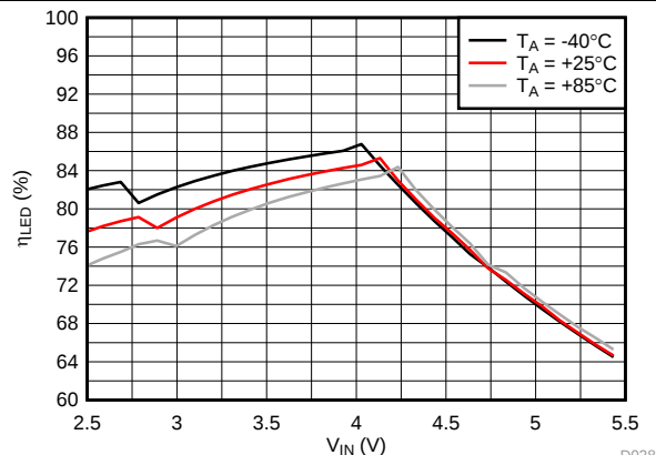
Figure 32. 2-MHz LED Efficiency vs Input Voltage
