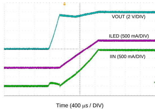
f_{SW} = 2 \text{ MHz} V_{LED} = 3.18 \text{ V} Brightness Code = 0x7F
