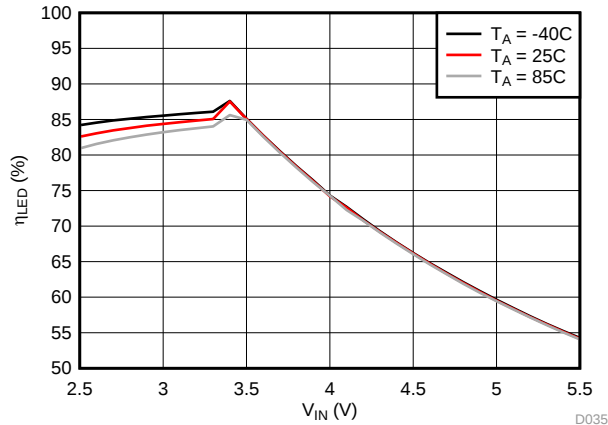
LM3648TT f_{SW} = 4 \text{ MHz} Torch Brightness Code = 0x59 V_{LED} = 3.03 \text{ V}
