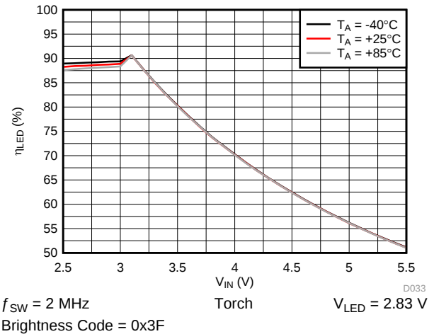
Figure 37. LED Efficiency vs Input Voltage
