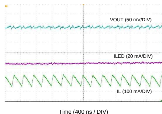
f_{SW} = 4 \text{ MHz} V_{LED} = 3.18 \text{ V} Brightness Code = 0x7F
