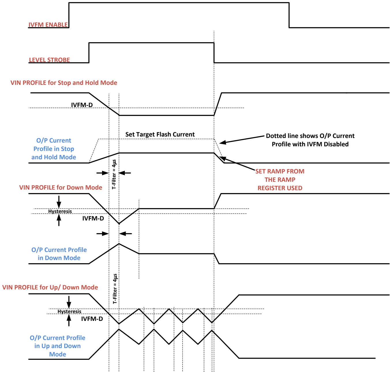
Figure 25. IVFM Modes
