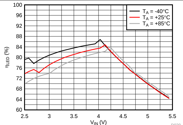
Figure 33. 4-MHz LED Efficiency vs Input Voltage
