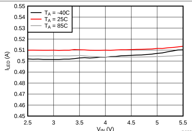
Figure 9. LED Current vs Input Voltage
