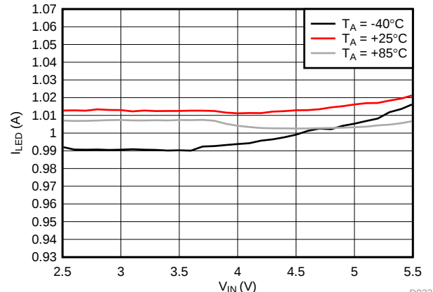
Figure 7. LED Current vs Input Voltage
