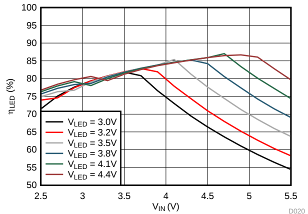
Figure 33. 4-MHz LED Efficiency vs Input Voltage
