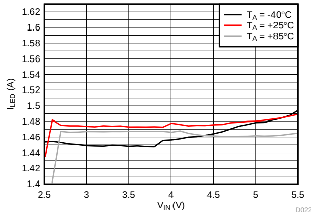
Figure 6. LED Current vs Input Voltage
