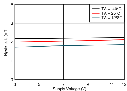
Figure 7-24. Hysteresis vs V_{CC}
