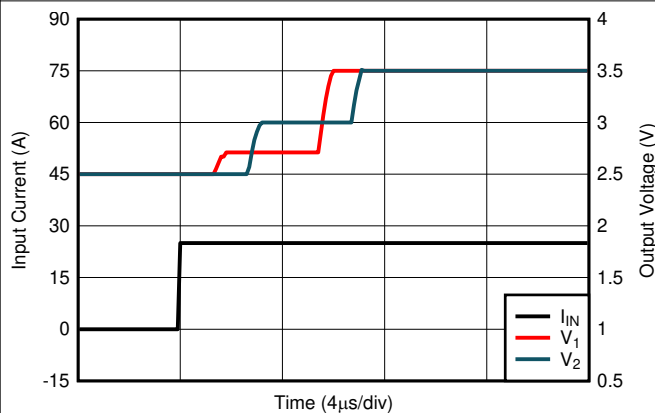
Figure 7-9. Voltage Output Step, Rising
