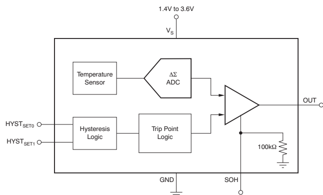
TMP303 Functional Block Diagram
