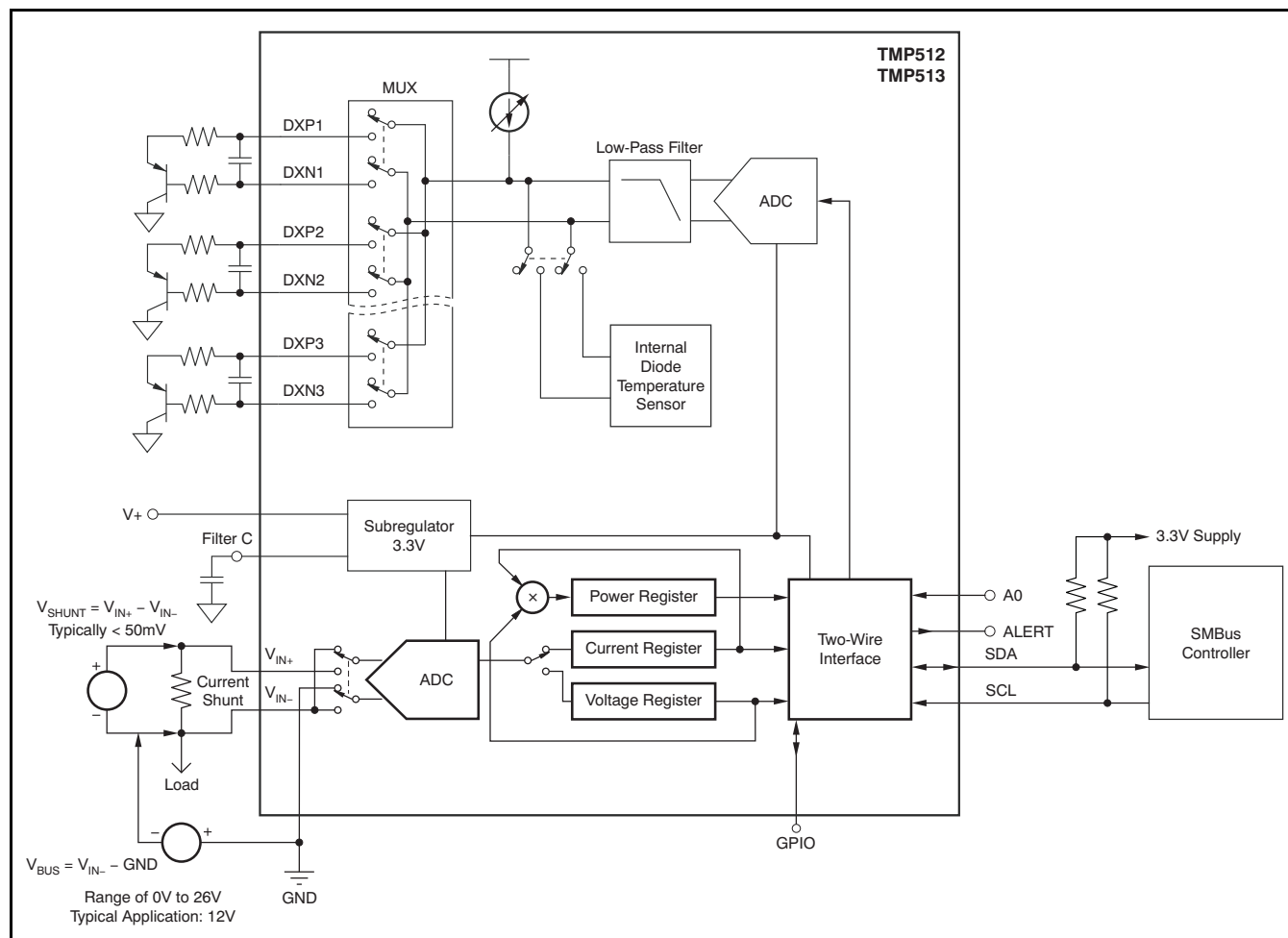
Figure 29. TMP512/13 Configured for Shunt and Bus Voltage Measurement
