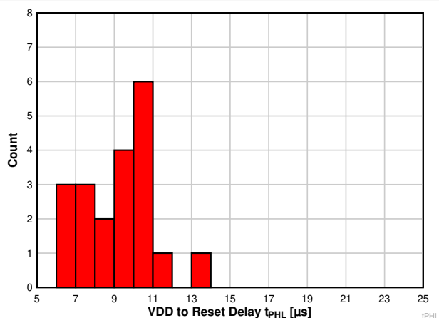
Figure 7-17. VDD to Reset Delay Histogram for TPS3823A-33 Devices at 125°C (Unit Count = 20)
