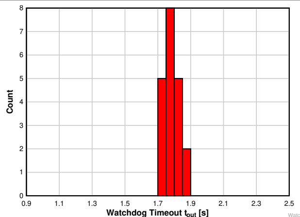
Figure 7-14. Watchdog Timeout Histogram for TPS3823A-33 Devices at 125°C (Unit Count = 20)
