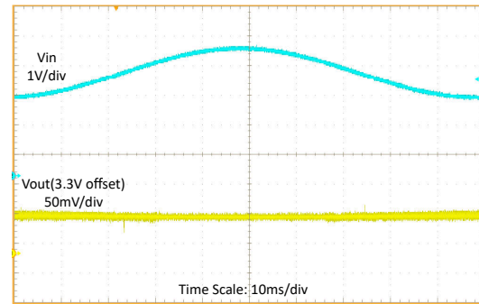
Figure 9-20. Line Sweep at 1-A Load Current
