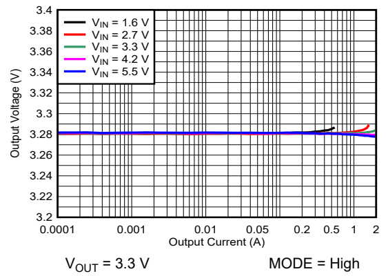
Figure 9-4. Load Regulation (FPWM)
