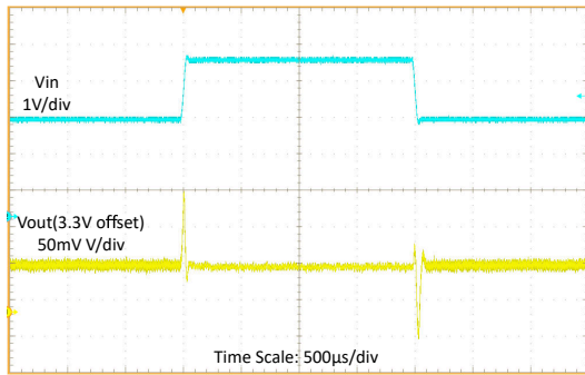
Figure 9-19. Line Transient at 1-A Load Current
