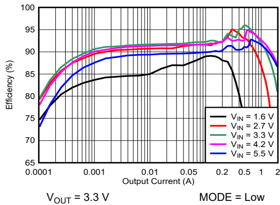
Figure 9-5. Efficiency vs Input Voltage (PFM)
