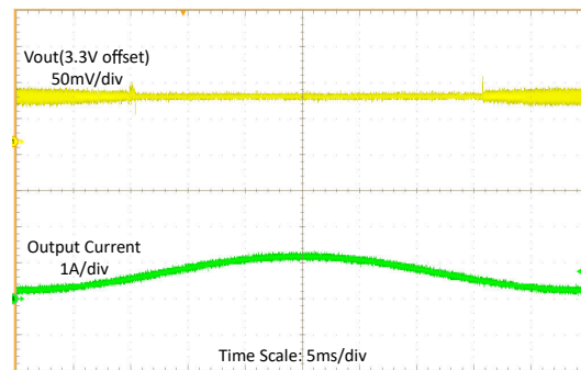
Figure 9-18. Load Sweep at 4.3-V Input Voltage
