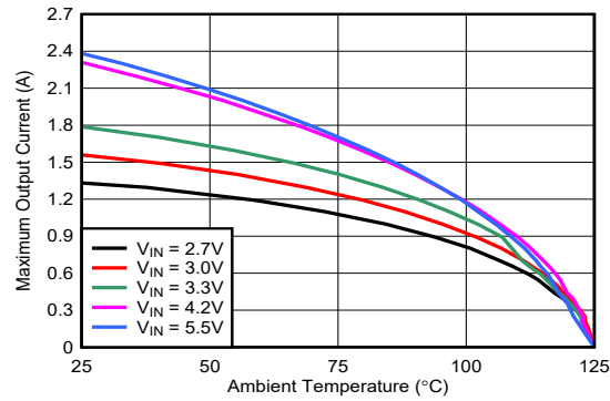
Figure 9-2. Safe Operating Area Based on Thermal Limitation
