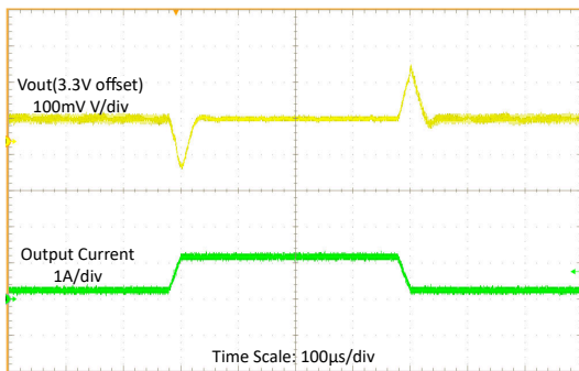
Figure 9-15. Load Transient at 3.6-V Input Voltage
