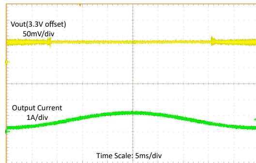
Figure 9-16. Load Sweep at 3.6-V Input Voltage
