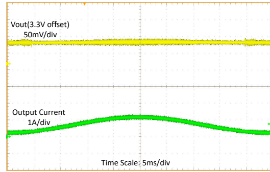
Figure 9-14. Load Sweep at 2.7-V Input Voltage
