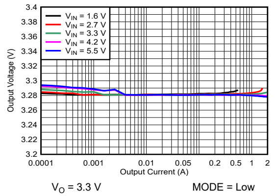
Figure 9-6. Load Regulation (PFM)
