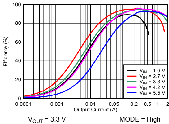
Figure 9-3. Efficiency vs Output Current (FPWM)
