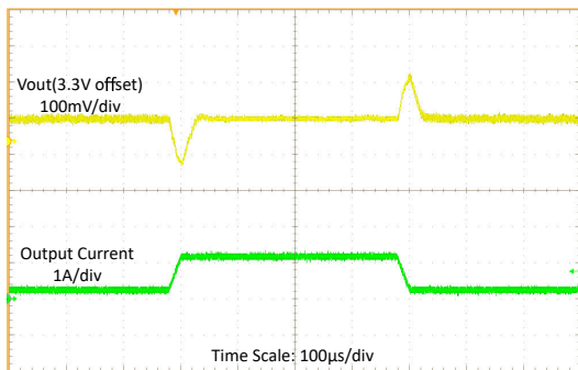
Figure 9-13. Load Transient at 2.7-V Input Voltage
