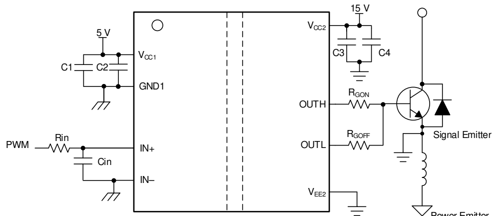
Figure 9-1. Typical Application Circuit for UCC5350SB-Q1 to Drive IGBT
