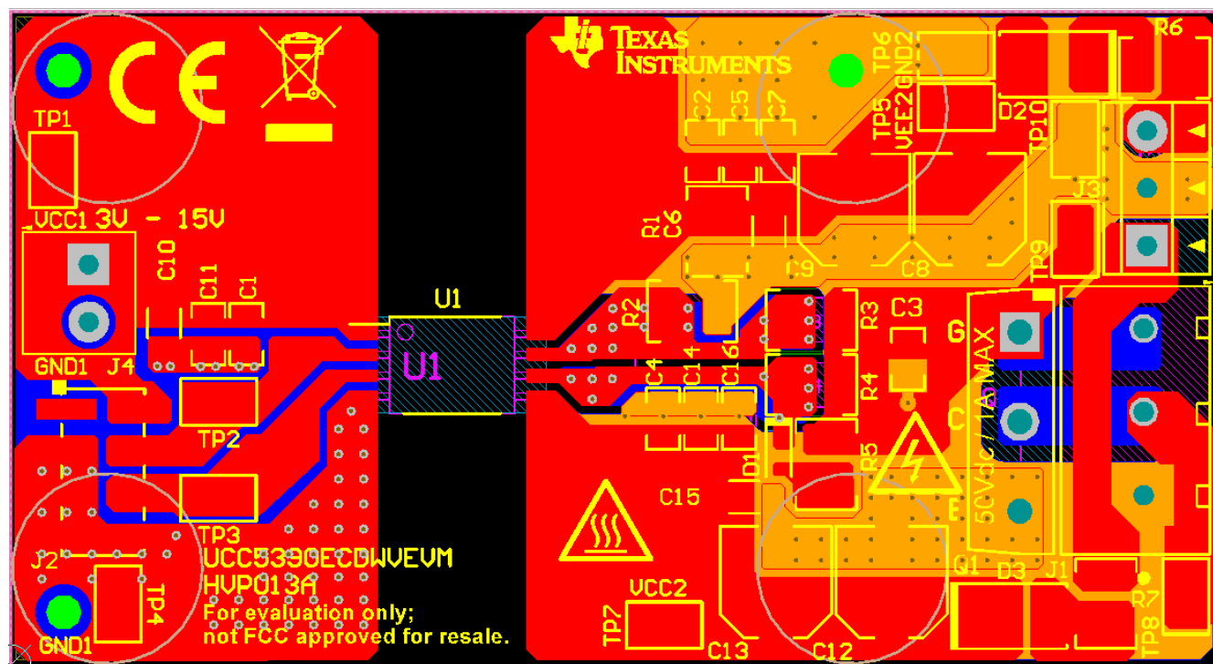
Figure 11-1. Layout Example
