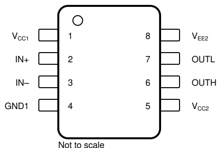
Figure 5-2. UCC5350SB-Q1 8-Pin SOIC Top View
