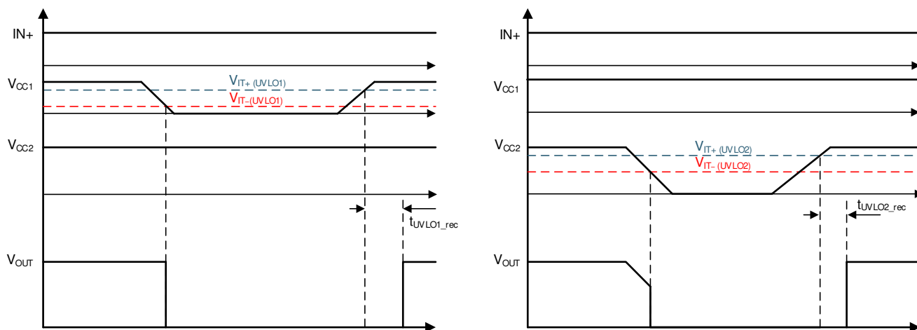
Figure 8-9. UVLO Functions
